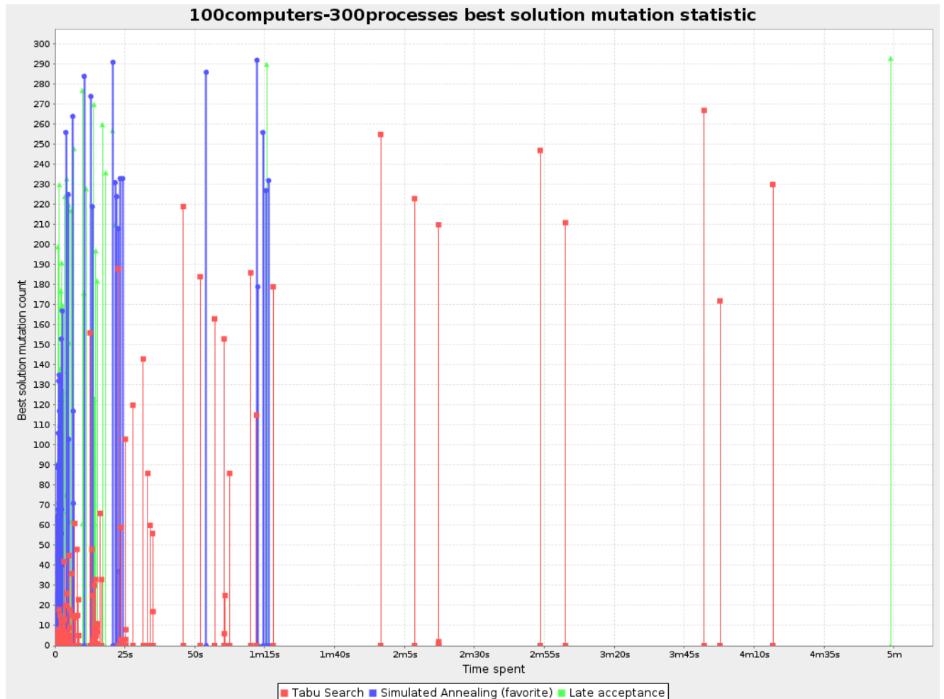
Figure 14.5. Best Solution Mutation Over Time Statistic
