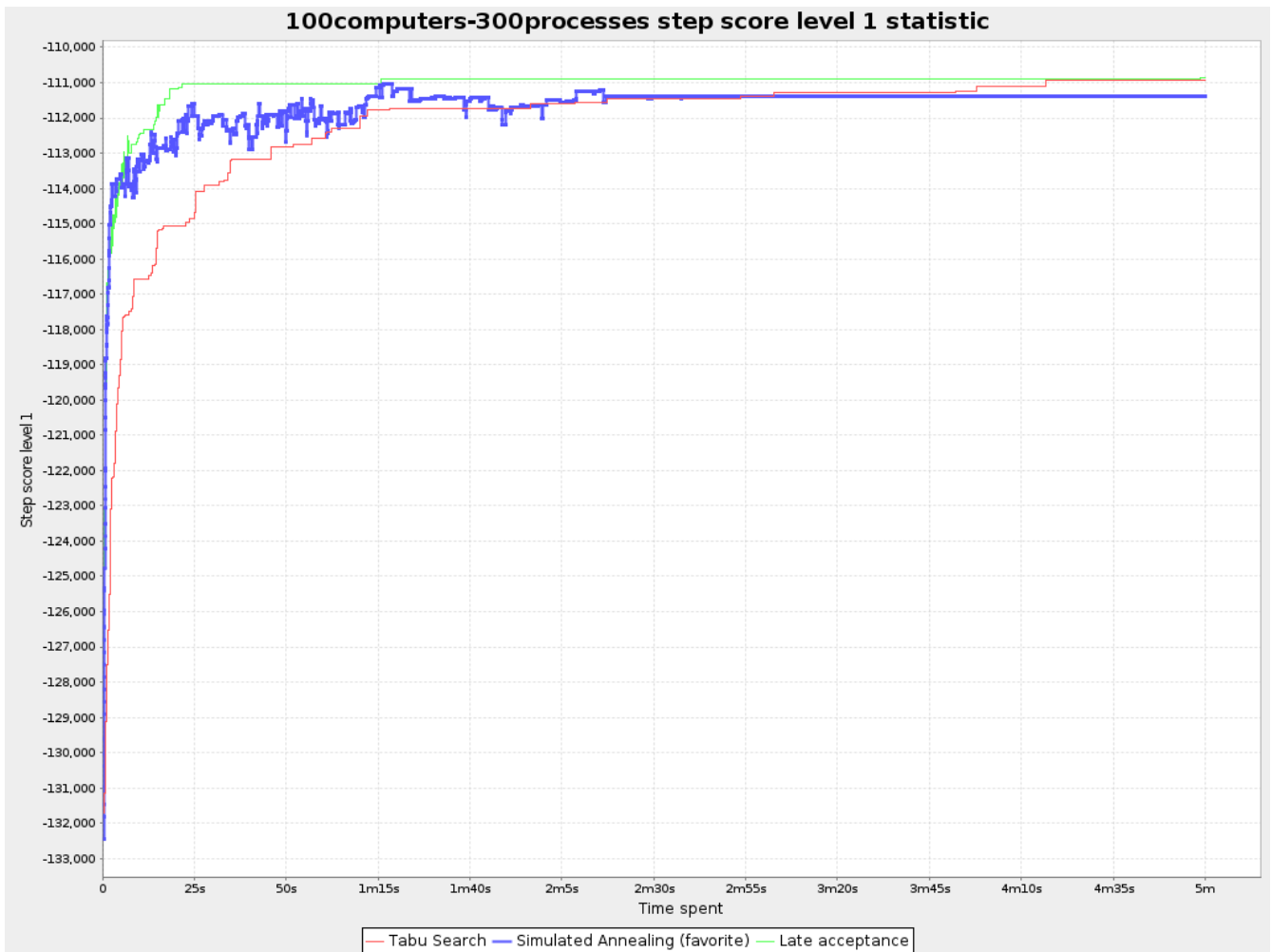
Figure 12. Step Score Over Time Statistic
